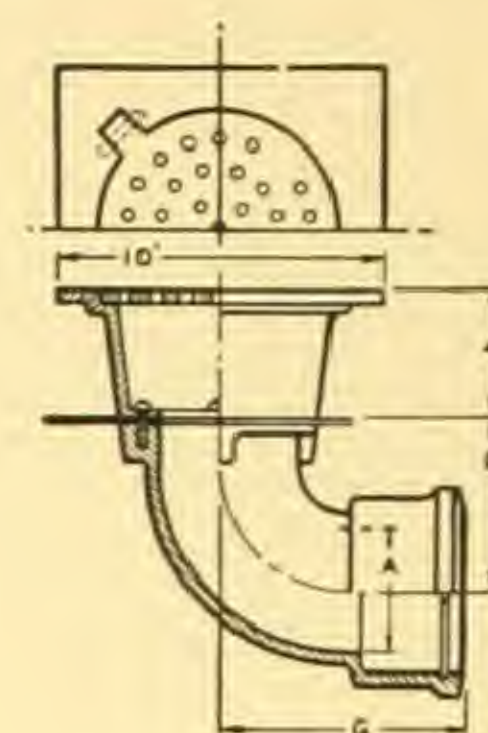
Z-556A—Hub Outlet
