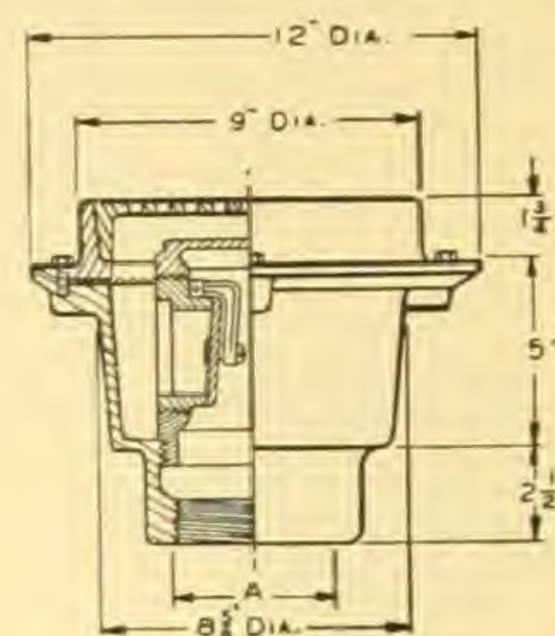
Z-511-1—I.P.S. Outlet
